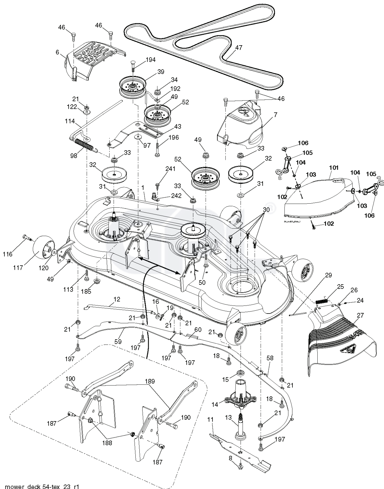
mower_deck 54-tex_23_r1
