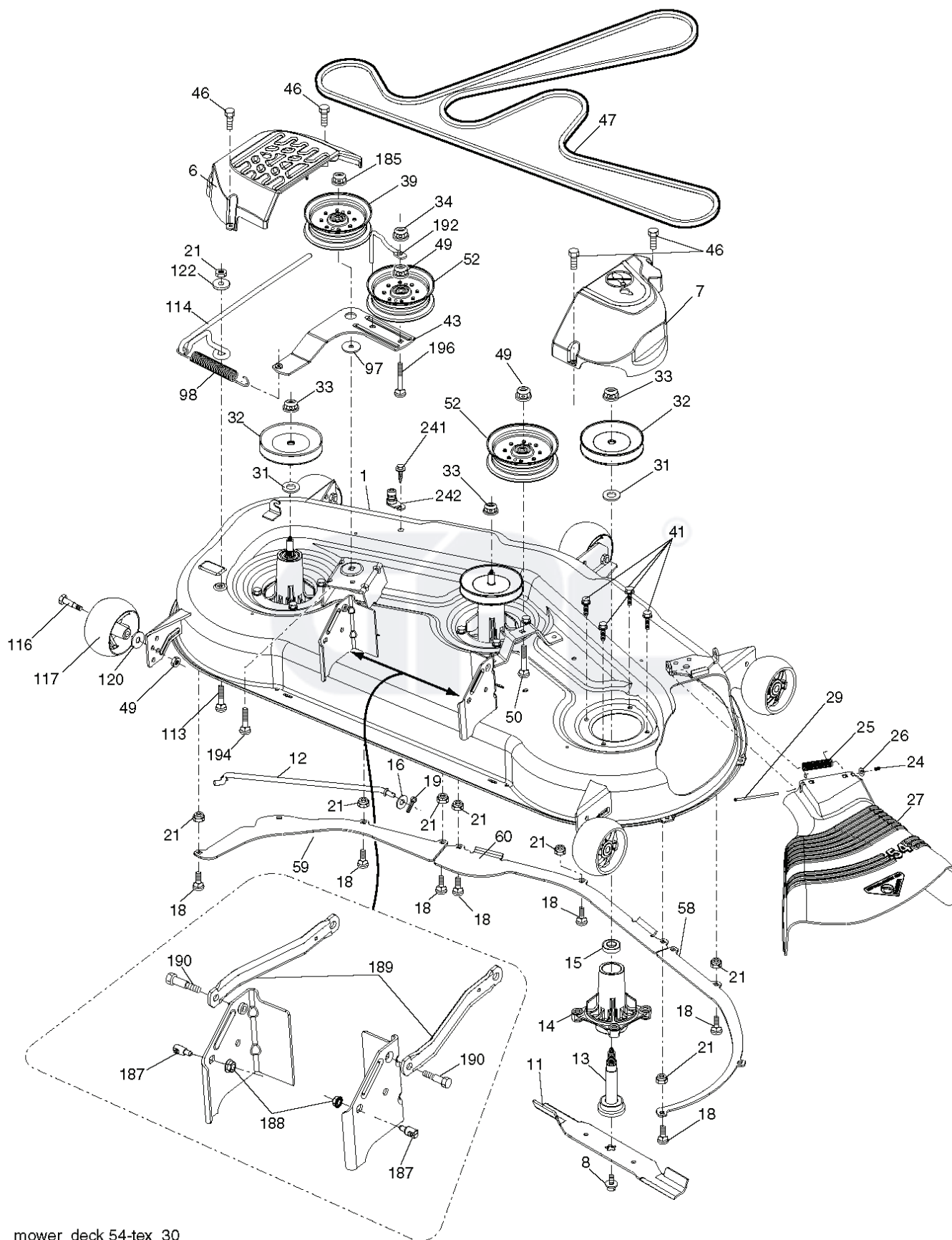
mower_deck 54-tex_30
