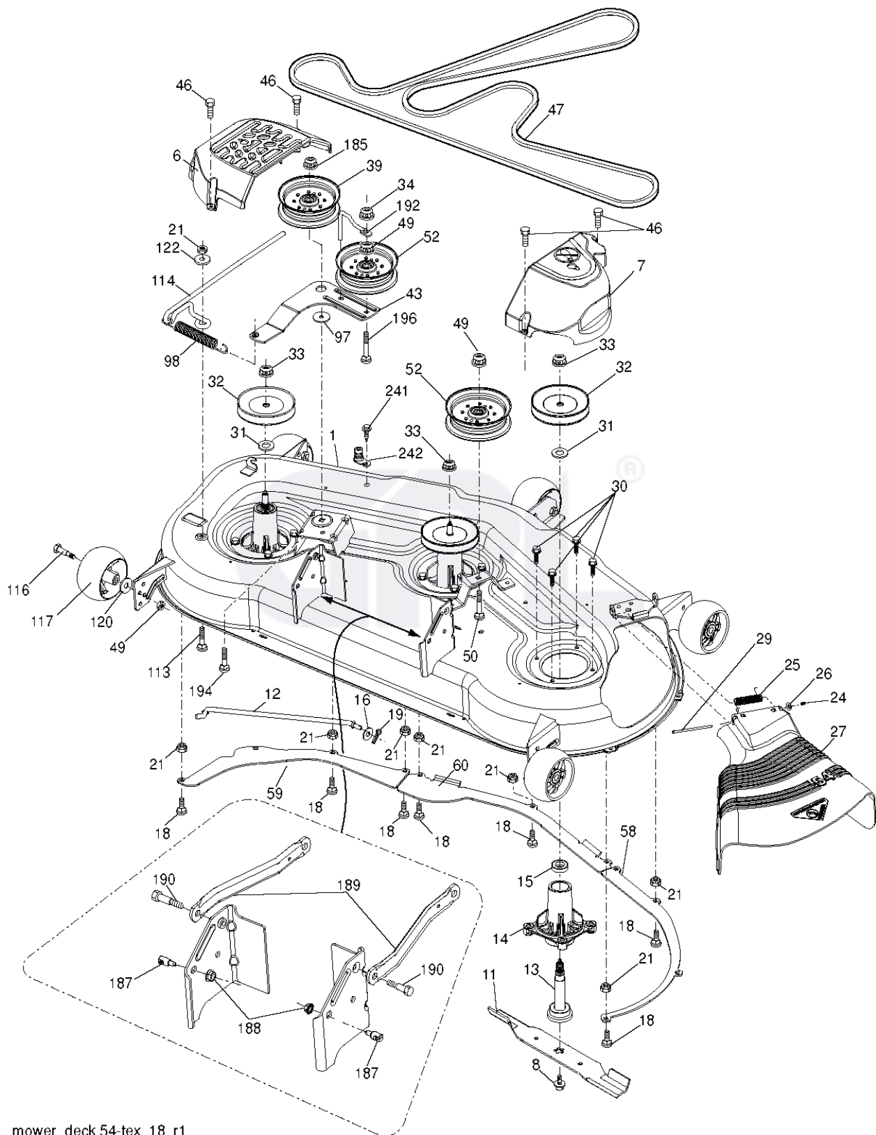
mower_deck 54-tex_18_r1
